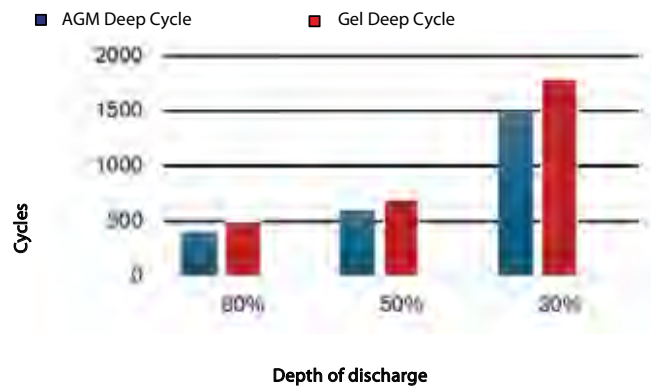
Fig. 2: Cycle life
