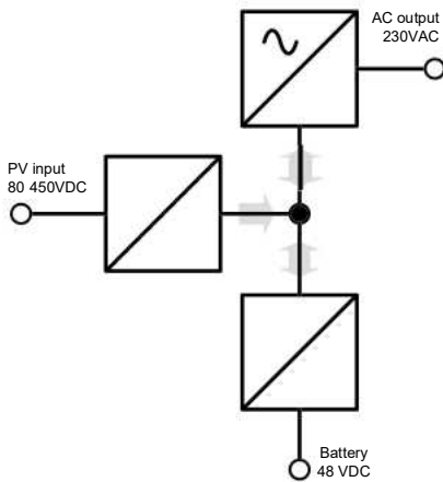
Inside the Inverter RS 48V
