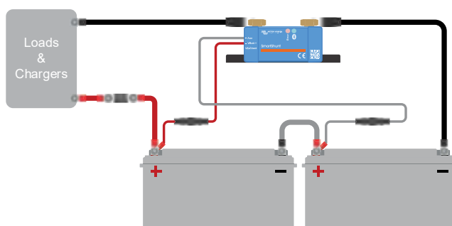
Measuring battery bank midpoint
